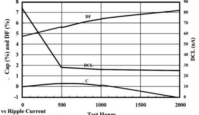
Life Test, 105 °C, Full Load, 330 μF, 400 V
