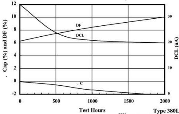
Life Test, 105 °C, Full Load, 120 μF, 400 V
