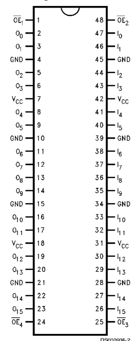
Pin Assignment for CERPAC
