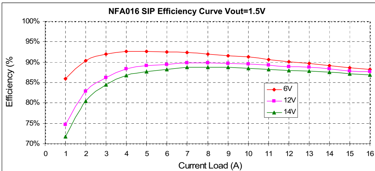
Fig 23. SIP Efficiency Curves for Vout=1.5V (25C)
