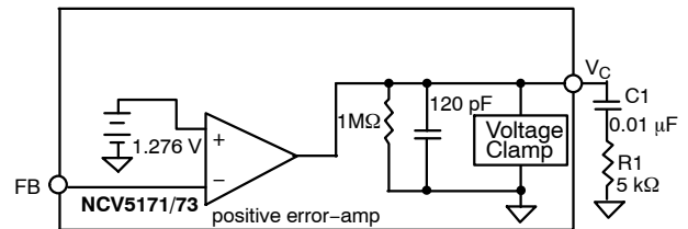
Figure 24. Error Amplifier Equivalent Circuit
