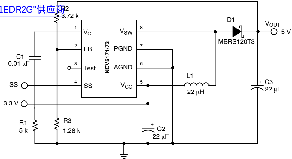
Figure 1. Applications Diagram
