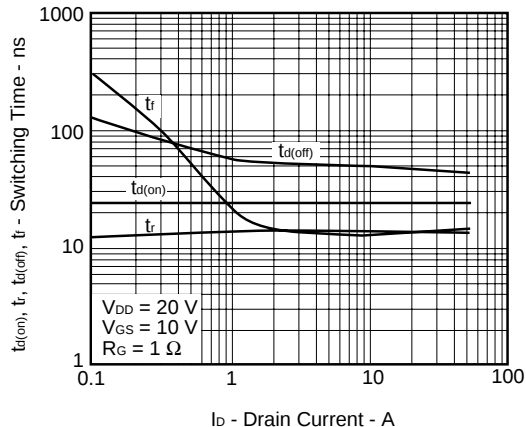
Figure15. SWITCHING CHARACTERISTICS
