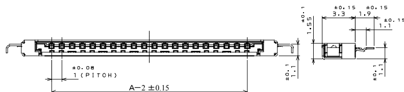
Diagram of connector when mated
