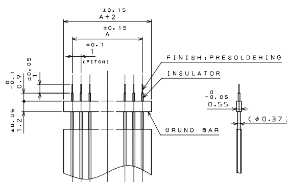
Diagram of connector when mated
