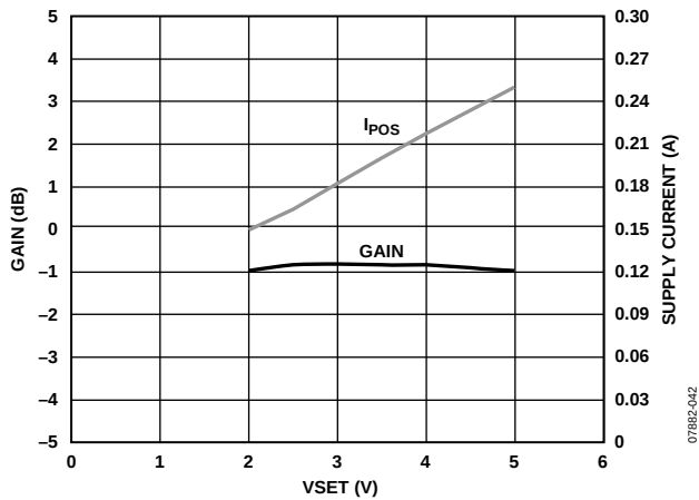
Figure 42. Power Conversion Gain and I_{POS} vs. VSET
