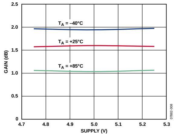
Figure 8. Power Conversion Gain vs. Supply Voltage
