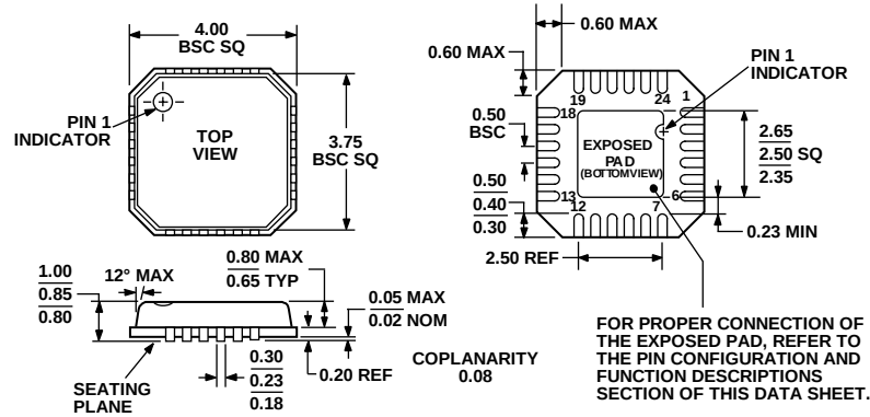
Figure 76. 24-Lead Lead Frame Chip Scale Package [LFCSP_VQ] 4 mm x 4 mm Body, Very Thin Quad (CP-24-3) Dimensions shown in millimeters
