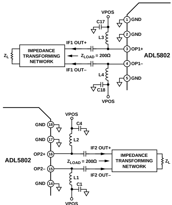
Figure 72. Biasing the IF Port Open-Collector Outputs Using Pull-Up Choke Inductors
