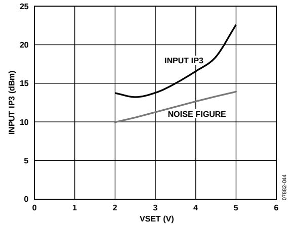
Figure 44. Input IP3, Noise Figure vs. VSET
