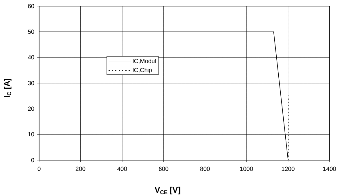
Reverse bias safe operating area Inverter (RBSOA) T_{vj} = 125^\circ C , V_{GE} = \pm 15V , R_G = 27 \text{ Ohm}
