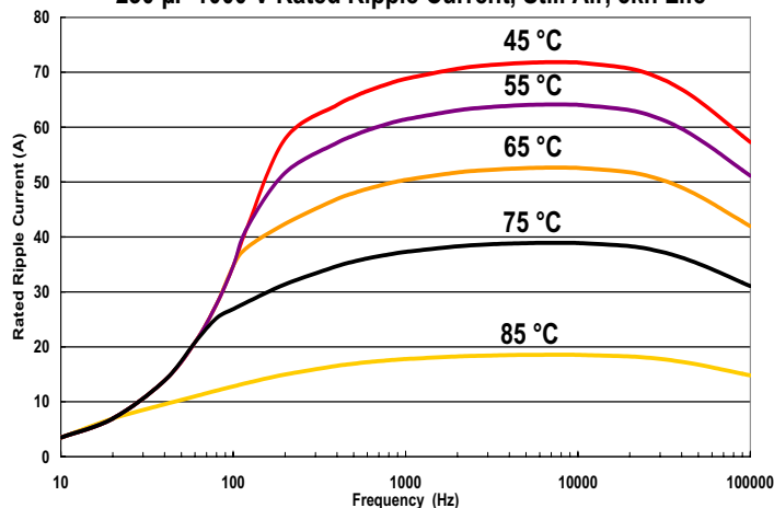
230 \mu F 1000 V Rated Ripple Current, Still Air, 5kh Life
