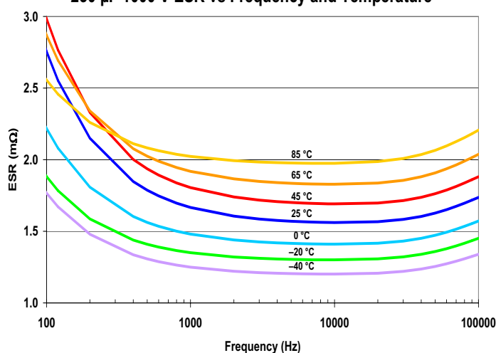
230 \mu F 1000 V ESR vs Frequency and Temperature
