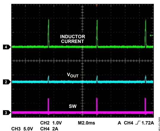
Figure 69. Hiccup Mode
