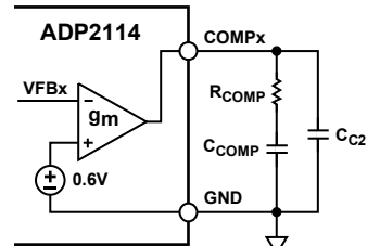
Figure 77. Compensation Components
