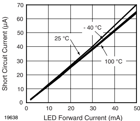
Fig. 3 - I_{SC} vs. LED Forward Current
