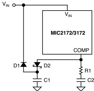
Figure 8. Soft Start
