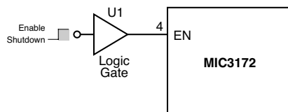
Figure 3. MIC3172 TTL Enable/Shutdown
