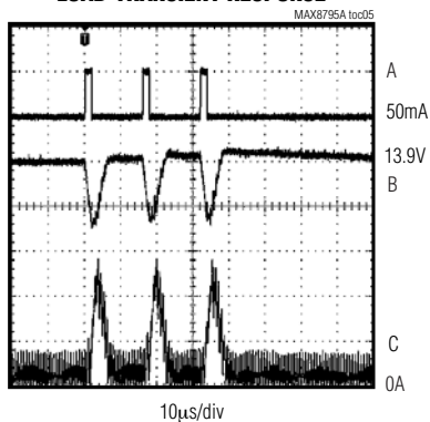
STEP-UP REGULATOR PULSED LOAD-TRANSIENT RESPONSE
