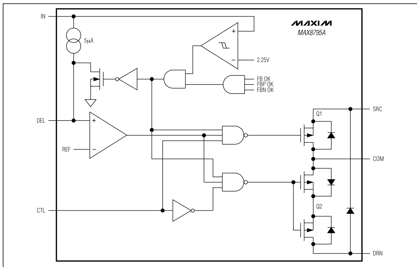
Figure 7. Switch-Control Block
