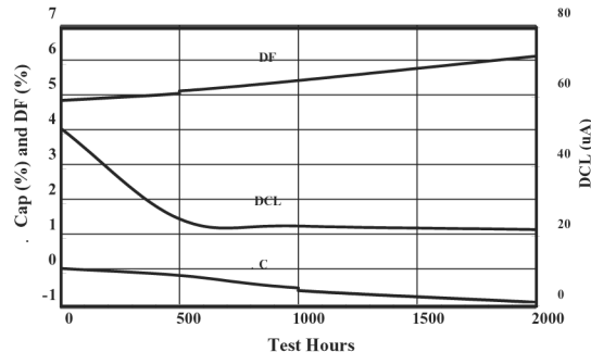
Life Test, 105 °C, Full Load, 330 \mu\text{F} , 400 V
