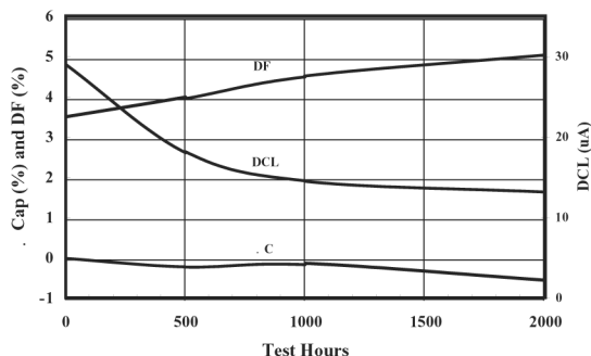
Life Test, 105 °C, Full Load, 220 \mu\text{F} , 400 V
