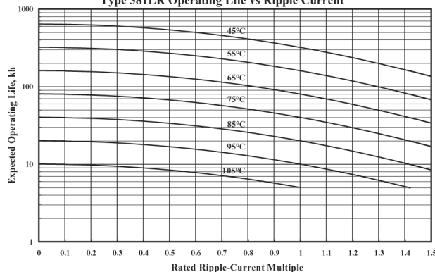
Type 381LR Operating Life vs Ripple Current
