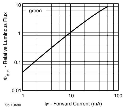
Figure 16. Relative Luminous Flux vs. Forward Current
