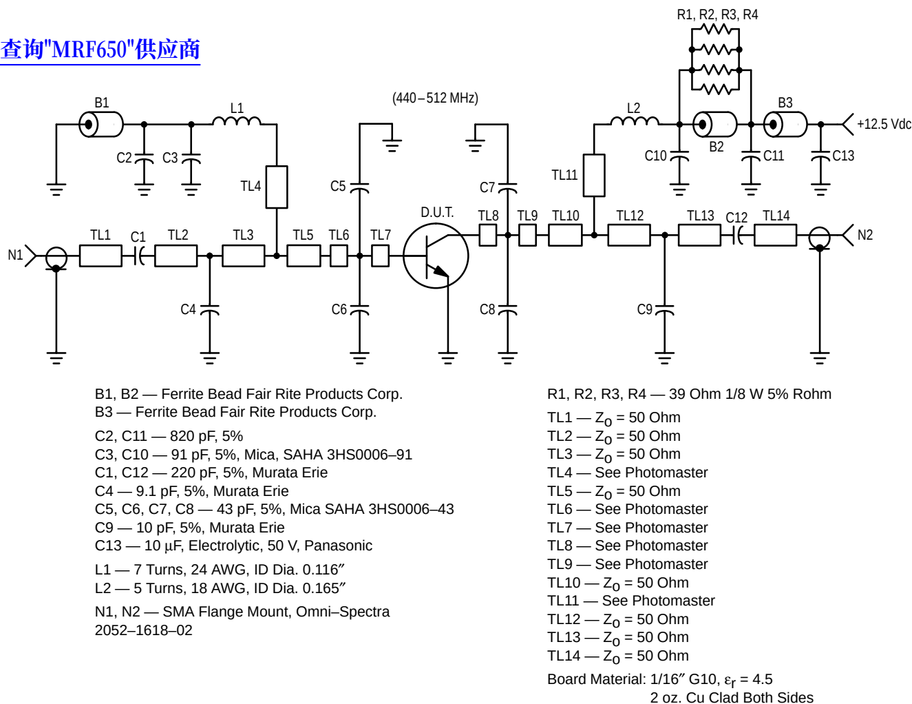
Figure 7. Schematic of Broadband Demonstration Amplifier (3)
