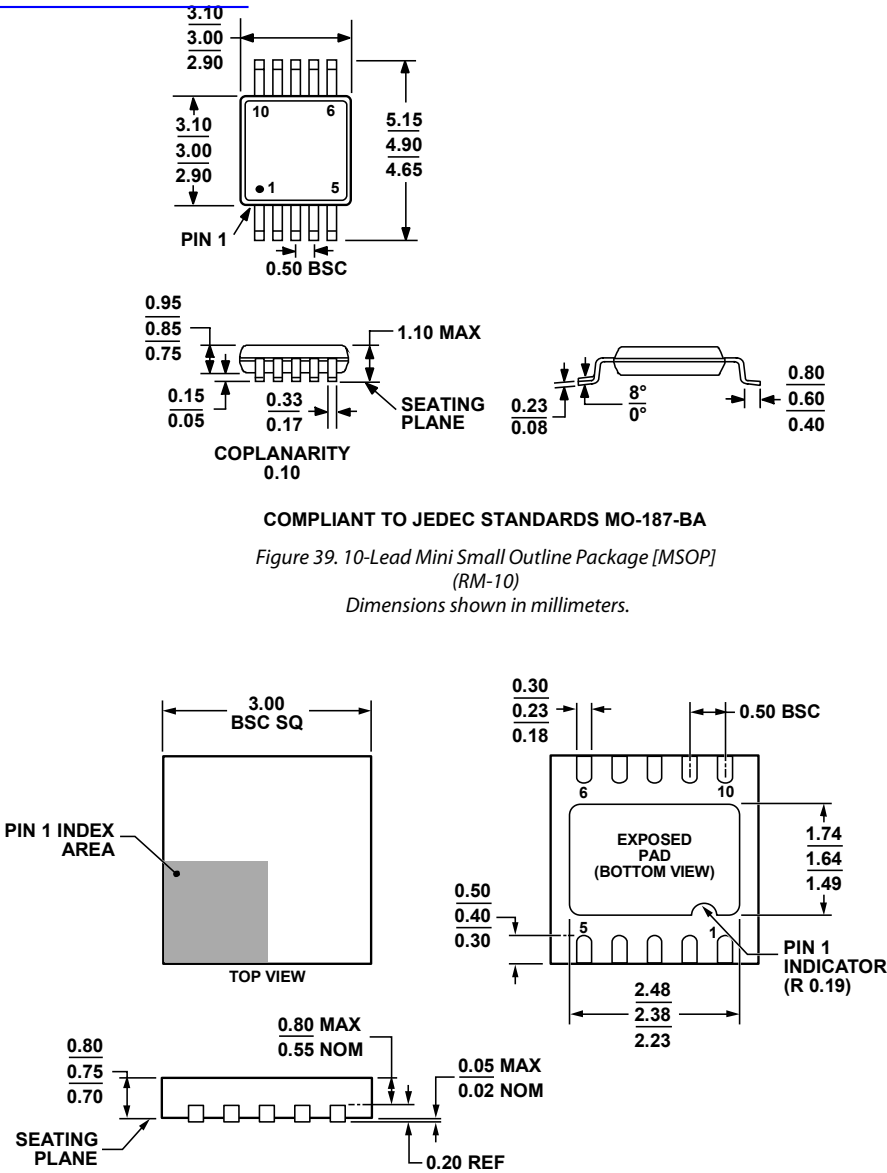
Figure 40. 10-Lead Lead Frame Chip Scale Package [LFCSP] (CP-10-9)
