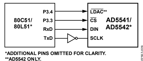
Figure 36. AD5541/AD5542 to 80C51/80L51 Interface
