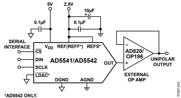
Figure 31. Unipolar Output
