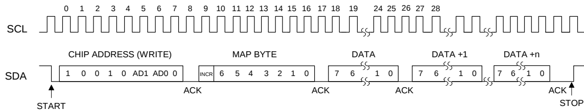
Figure 23. Control Port Timing, I²C Write
