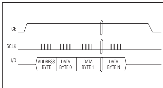
Figure 15. 3-Wire Multiple-Byte Burst Transfer
