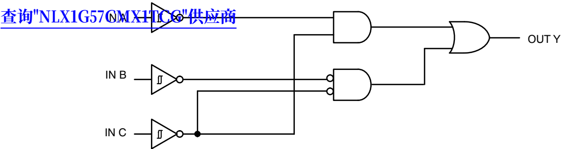
Figure 1. Function Diagram
