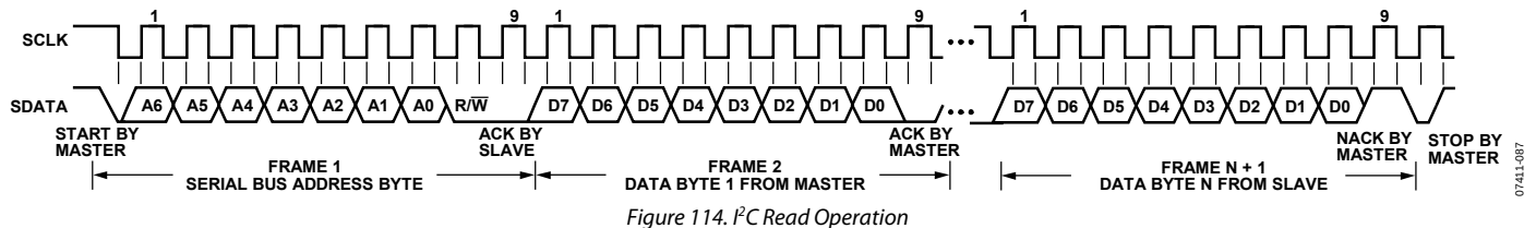
Figure 114. I 2 C Read Operation
