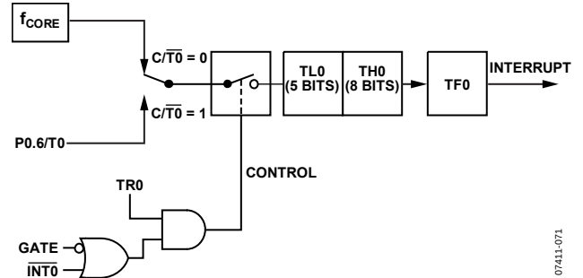
Figure 97. Timer/Counter 0, Mode 0
