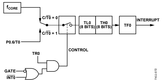
Figure 98. Timer/Counter 0, Mode 1
