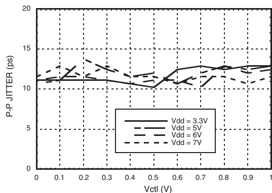
Peak-to-Peak Jitter vs. Vdd @ 11.25 Gbps [3][4]
