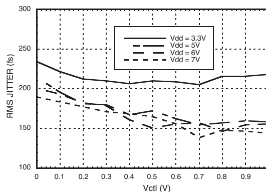
RMS Jitter vs. Vdd @ 22.5 Gbps [2]
