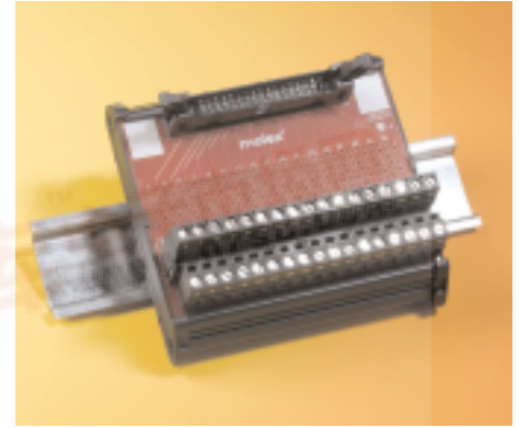
Ribbon-Cable module
