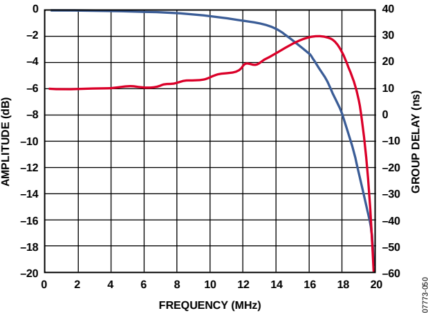
Figure 46. Low-Pass Chebyshev II Filter Response
