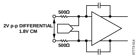
Figure 20. Equivalent Analog Input Circuit
