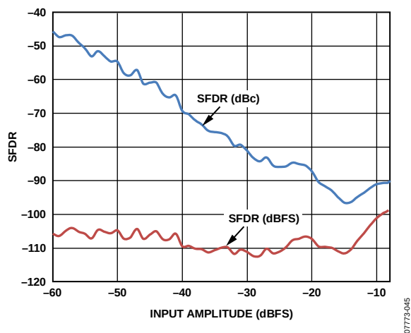
Figure 17. Two-Tone SFDR vs. Input Amplitude with f_{IN1} = 7.2 \text{ MHz} , f_{IN2} = 8.4 \text{ MHz}
