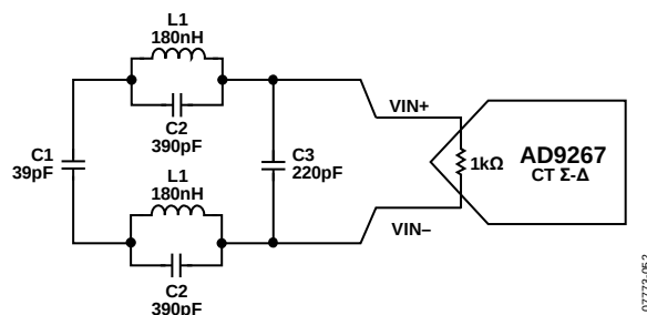
Figure 45. Third-Order Low-Pass Chebyshev II Filter
