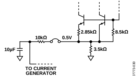
Figure 36. Internal Reference Configuration
