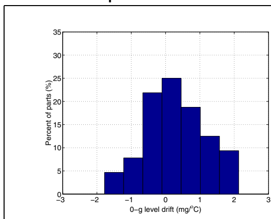
Figure 16. Y axis 0-g level change vs. temperature at 2.5V
