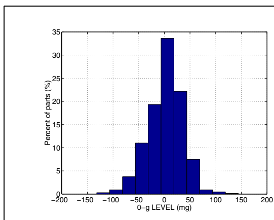
Figure 12. Y axis 0-g level at 2.5V
