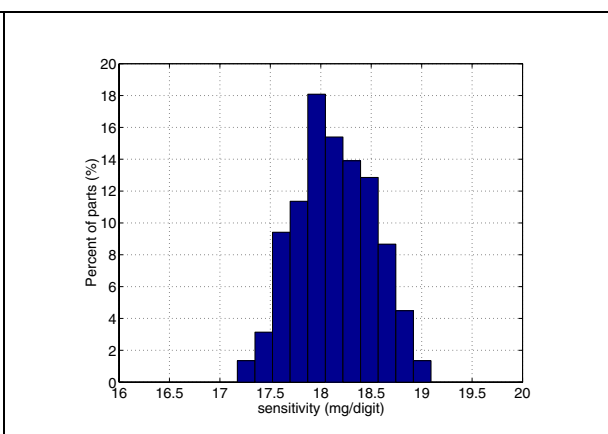
Figure 13. Y axis sensitivity at 2.5V
