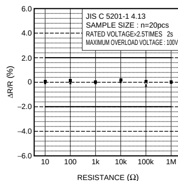
Fig.4 Overload
