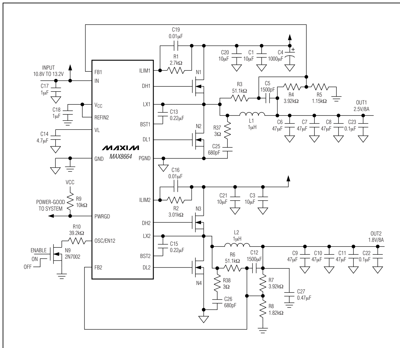
Figure 2. Low-Cost, 600kHz Typical Application Circuit
