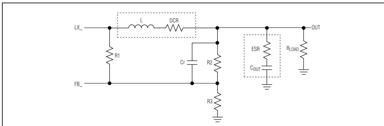
Figure 7. Feedback Network
