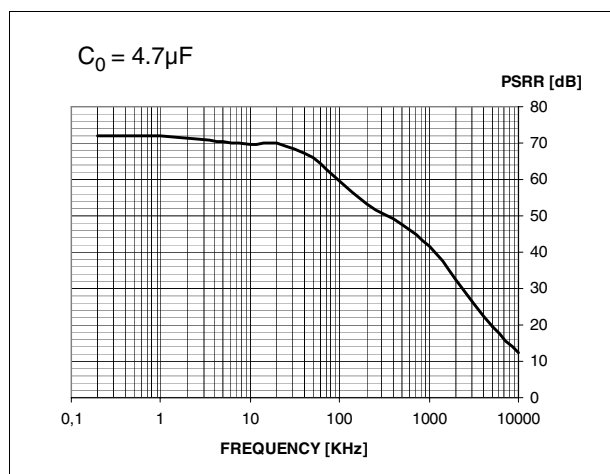
Figure 21. PSRR
