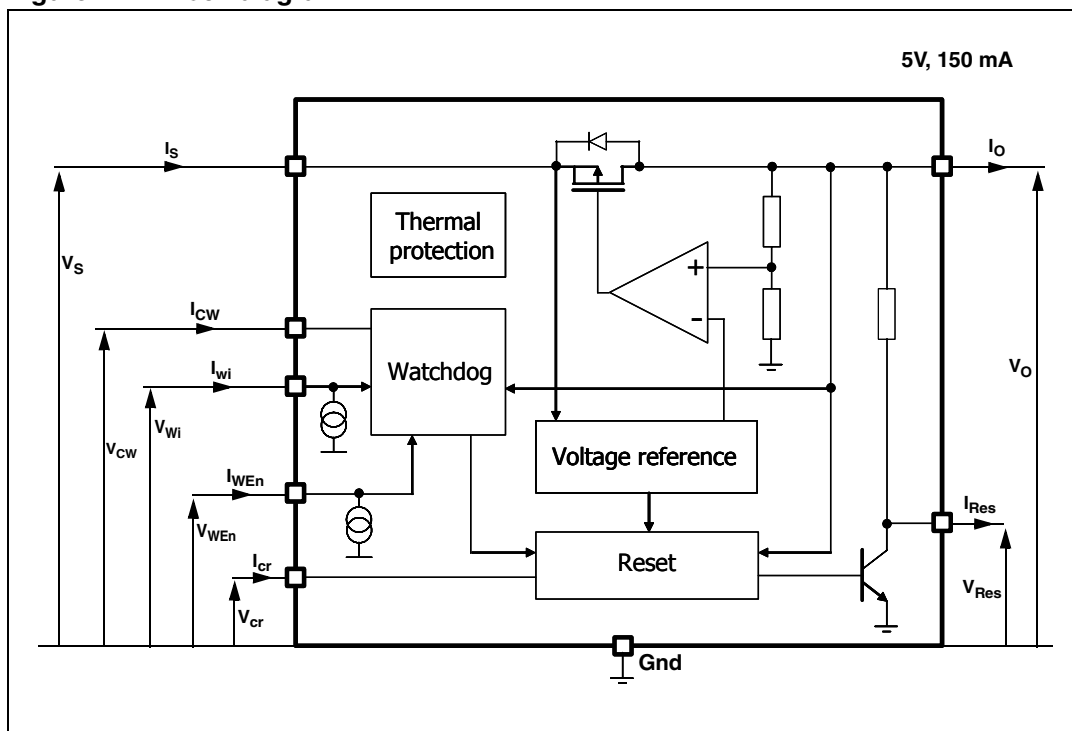
Figure 1. Block diagram
