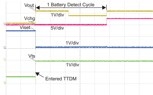
Figure 10. Battery Removal with OUT and TS Disconnect 1st, With 100- \Omega Load
