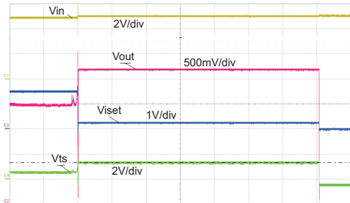
Figure 9. Battery Removal - GND Removed 1st, 42- \Omega Load
