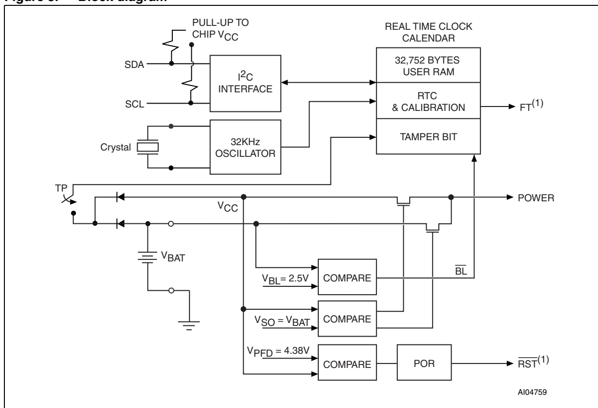
Figure 3. Block diagram
