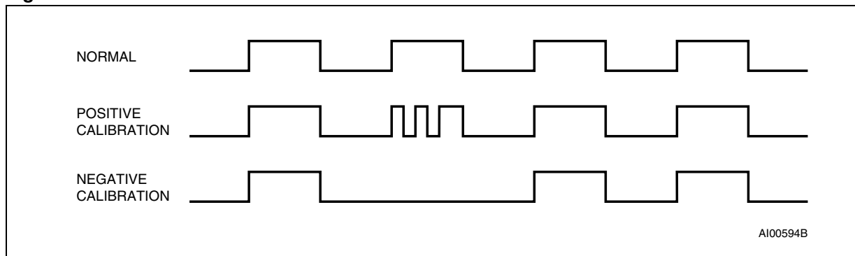
Figure 12. Clock calibration
