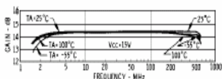
Gain
