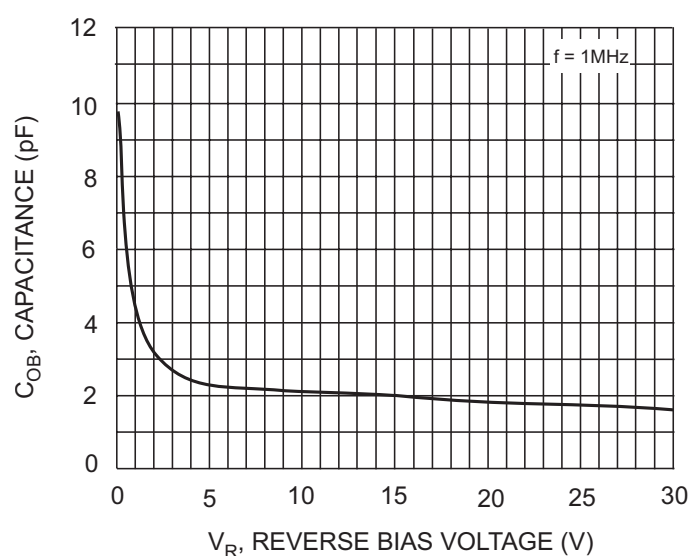
Fig. 4 Output Capacitance
