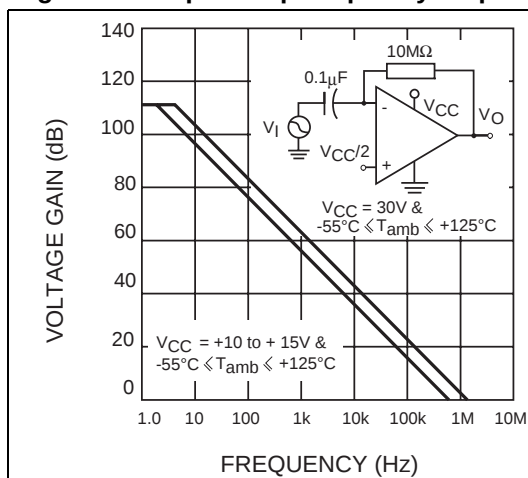
Figure 2. Open loop frequency response
