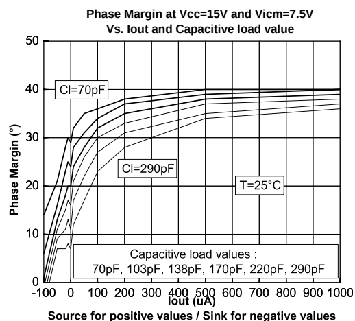
Figure 17. Phase margin vs capacitive load
