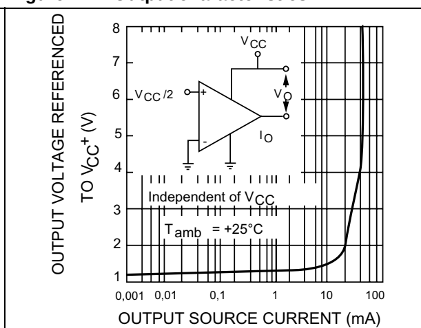
Figure 7. Output characteristics
