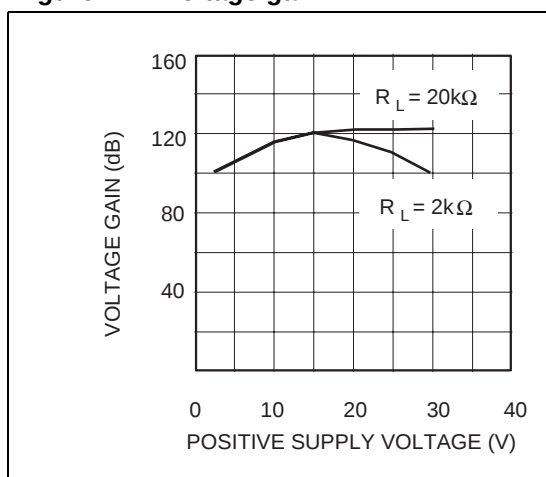
Figure 12. Voltage gain
