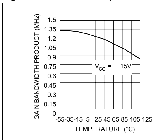
Figure 14. Gain bandwidth product
