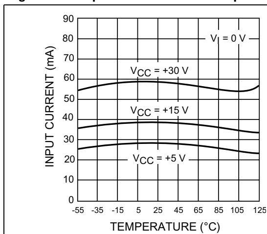
Figure 8. Input current versus temperature
