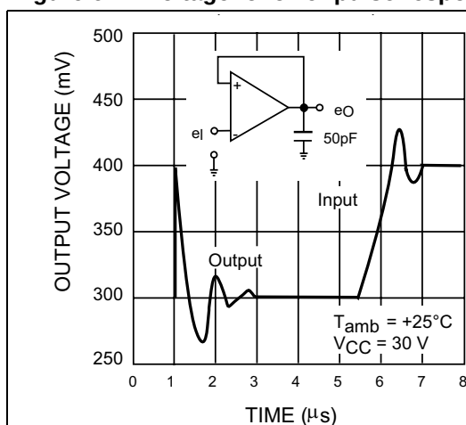
Figure 6. Voltage follower pulse response
