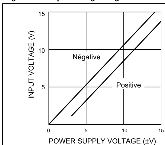
Figure 10. Input voltage range
