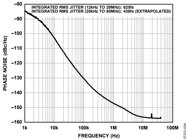
Figure 32. Phase Noise (Absolute) Clock Cleanup; Internal VCO @ 2177 MHz; PFD = 120 kHz; LBW = 1.92 kHz; LVDS Output = 155.52 MHz
