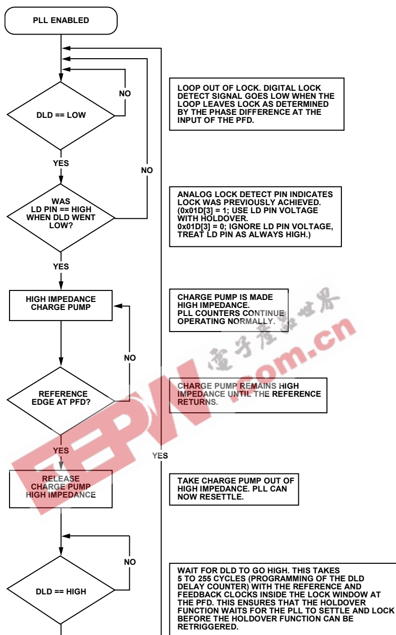
Figure 47. Flowchart of Automatic/Internal Holdover Mode
