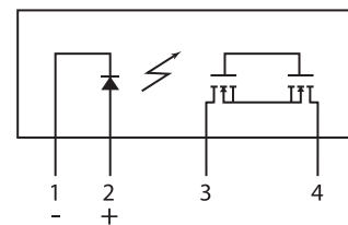
CPC1916Y Pinout
