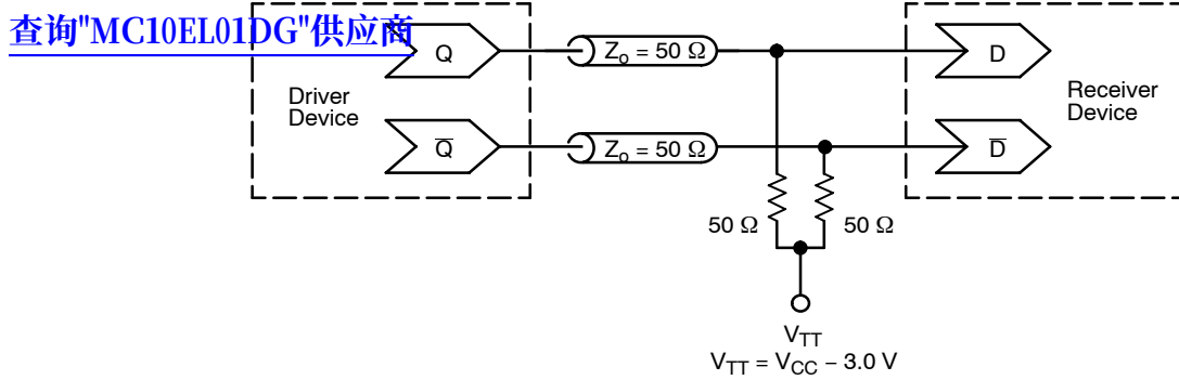
Figure 2. Typical Termination for Output Driver and Device Evaluation (See Application Note AND8020/D – Termination of ECL Logic Devices.)
