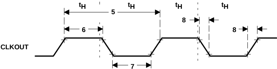
Figure 109. CLKOUT Timing
