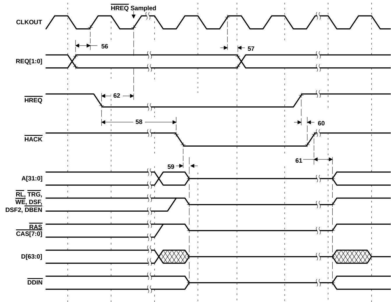
Figure 120. Host-Interface Timing
