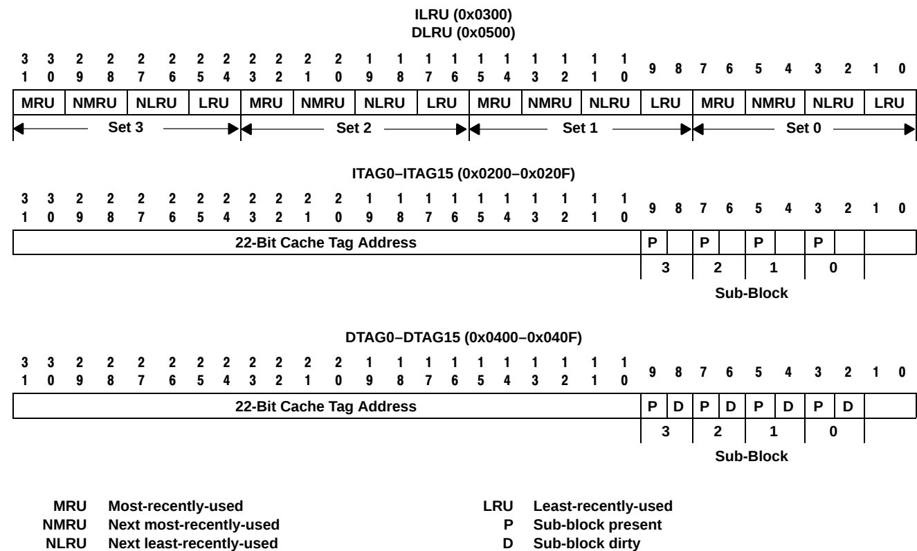
Figure 17. Cache Registers
