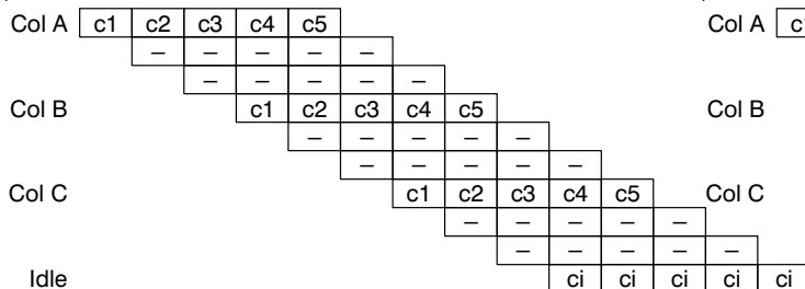
Figure 57. DRAM Cycle Column Pipelines
