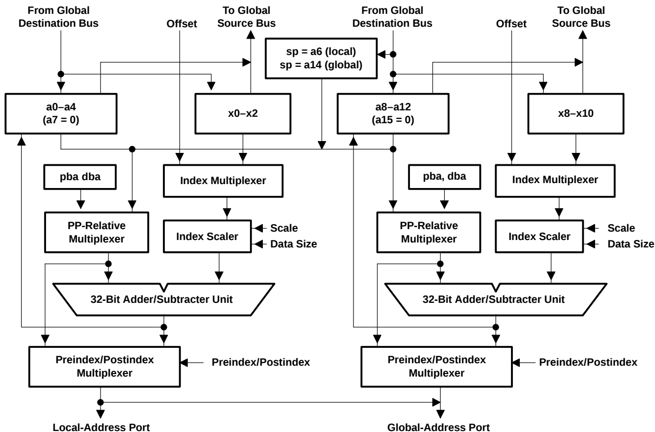
Figure 44. Address-Unit Architecture
