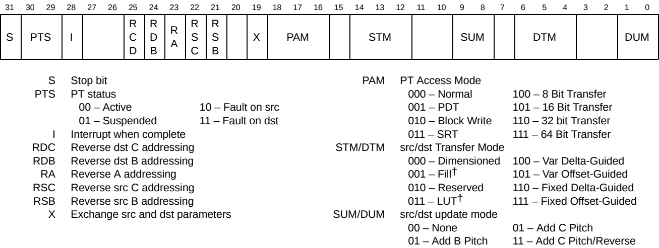
Figure 52. PT-Options Field
