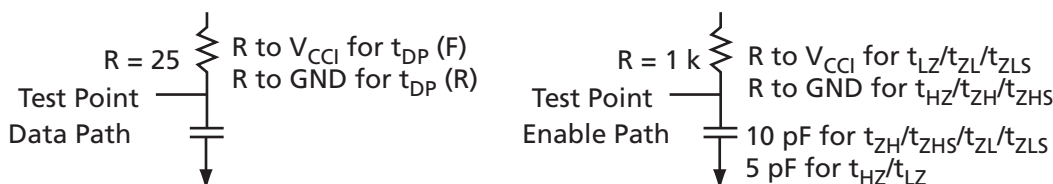
Figure 2-115 • AC Loading
