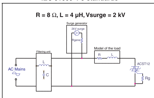
Figure 17. Overvoltage ruggedness test circuit for resistive and inductive loads for IEC 61000-4-5 standards
