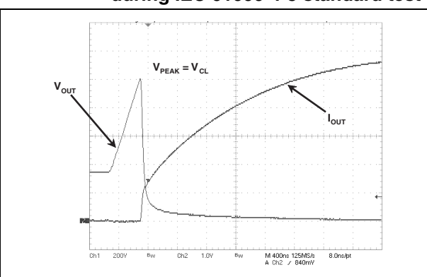
Figure 18. Typical current and voltage waveforms across the ACST10 during IEC 61000-4-5 standard test
