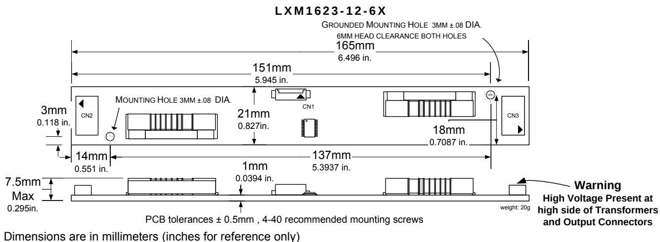
PHYSICAL DIMENSIONS
