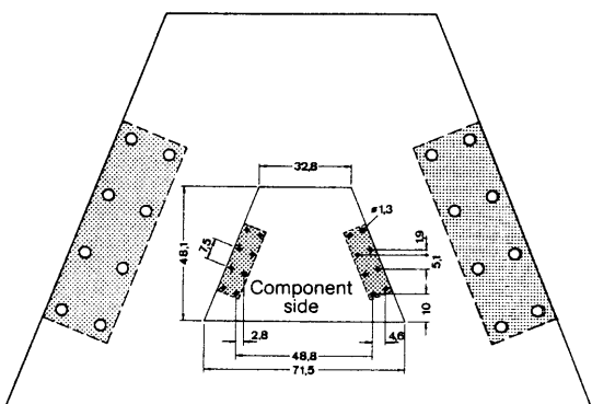
Printed Circuit Board for Component Housings with 3 Connection
