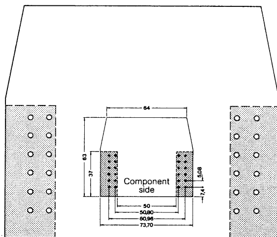
Printed Circuit Board P1-UEGM for Screw and Tab Connection
