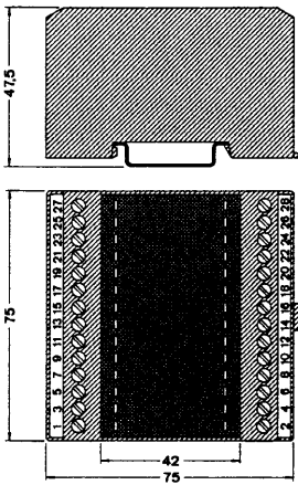
EMG 75 75 mm wide, 28 position
