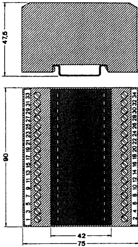
EMG 90 90 mm wide, 34 position
