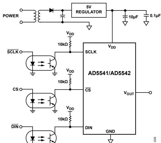
Figure 37. AD5541/AD5542 in an Optocoupler Interface
