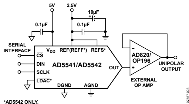
Figure 31. Unipolar Output
