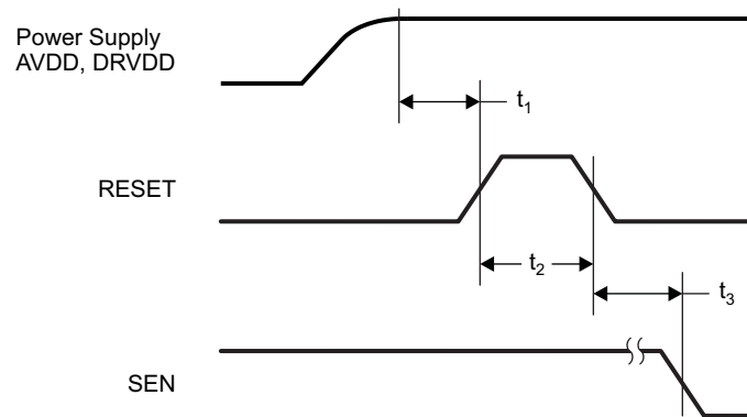
Figure 6. Reset Timing Diagram
