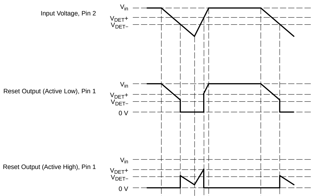
Figure 21. Timing Waveforms
