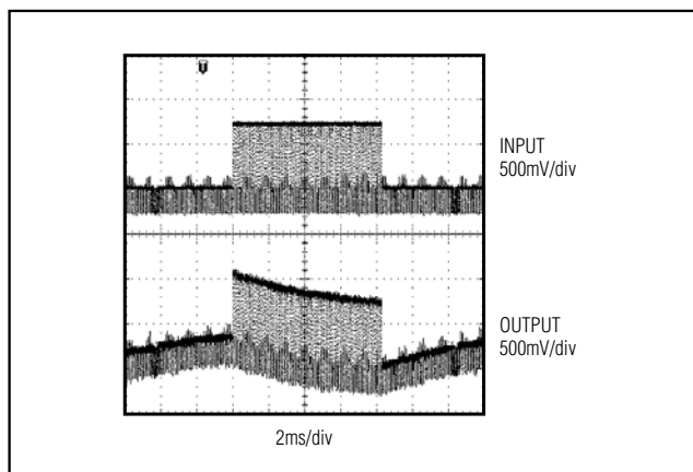
Figure 1. AC-Coupled Output
