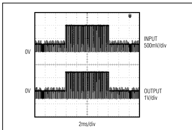
Figure 2. DirectDrive Output
