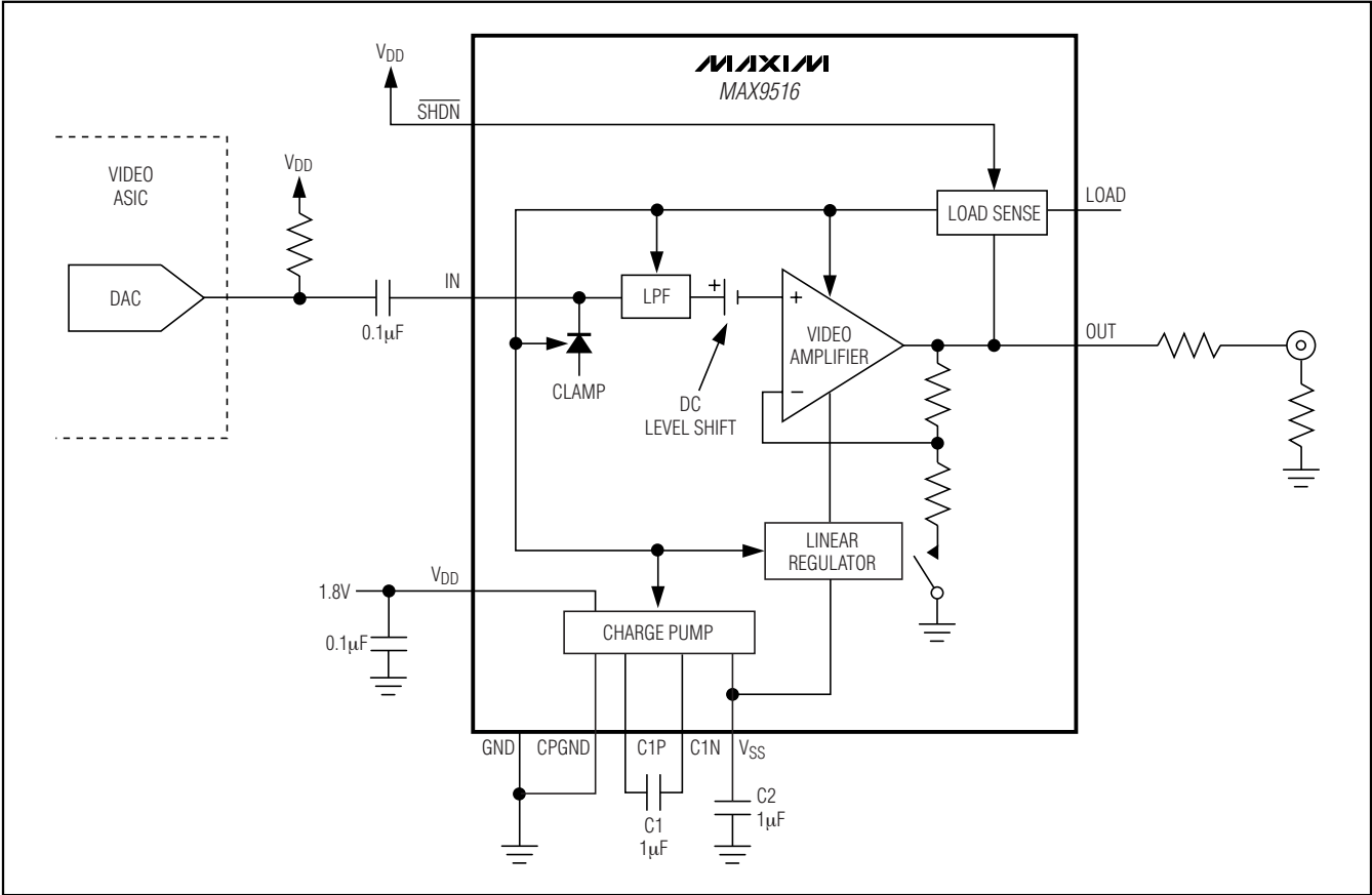
Figure 8. AC-Coupled Input
