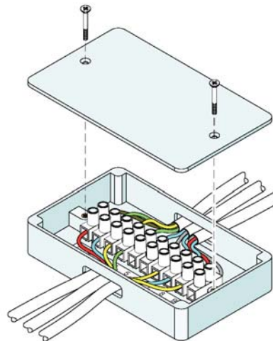
Junction Box
