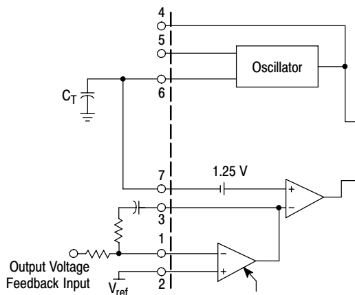
Figure 22. Voltage Mode Operation
