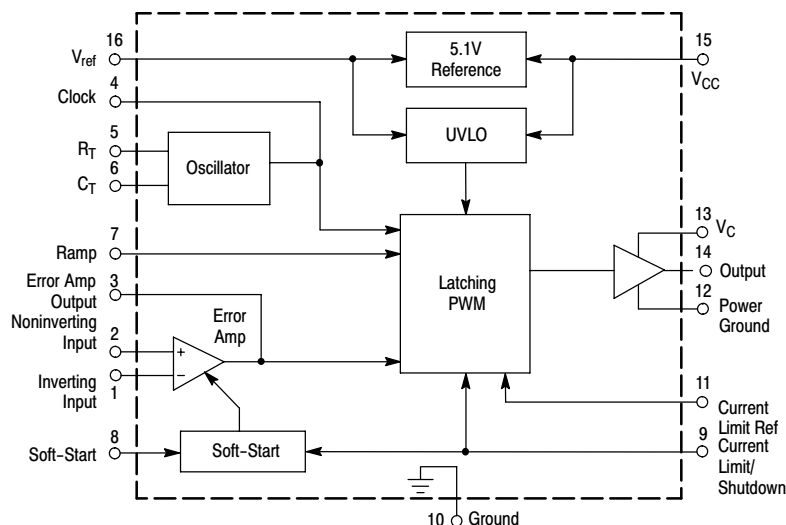
Figure 1. Simplified Application
