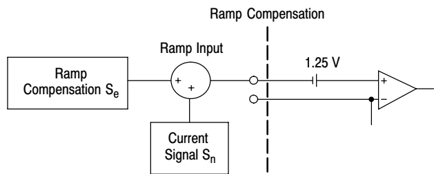
Figure 21. Ramp Compensation
