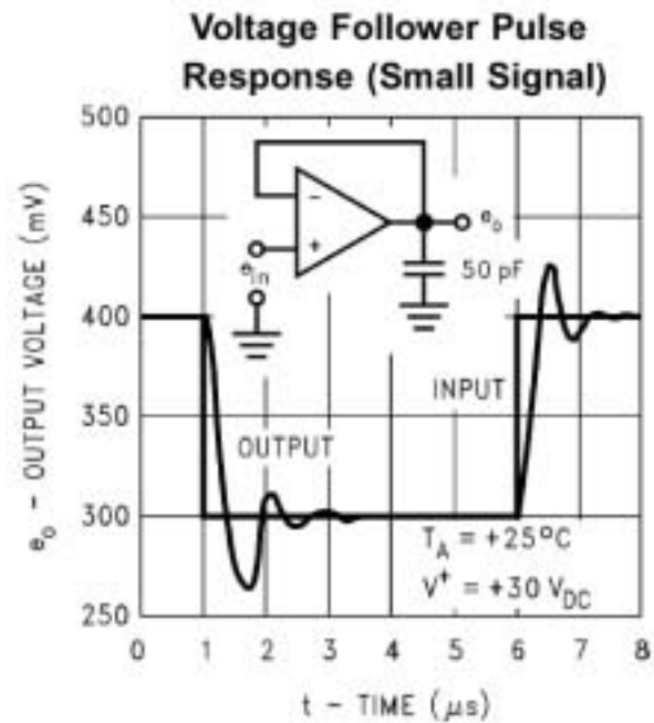
FIGURE 8. VOLTAGE FOLLOWER PULSE RESPONSE (SMALL SIGNAL)
