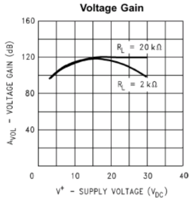
FIGURE 4. VOLTAGE GAIN
