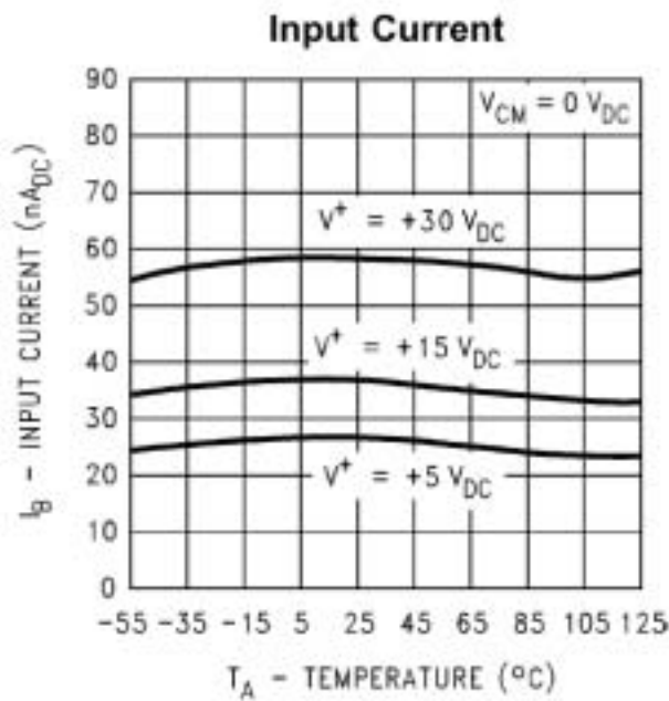
FIGURE 2. INPUT CURRENT
