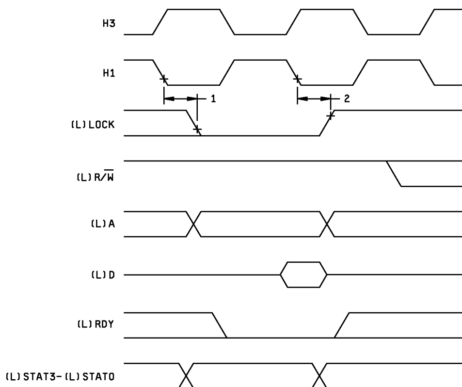
TIMING FOR (L) LOCK WHEN EXECUTING SIGI
