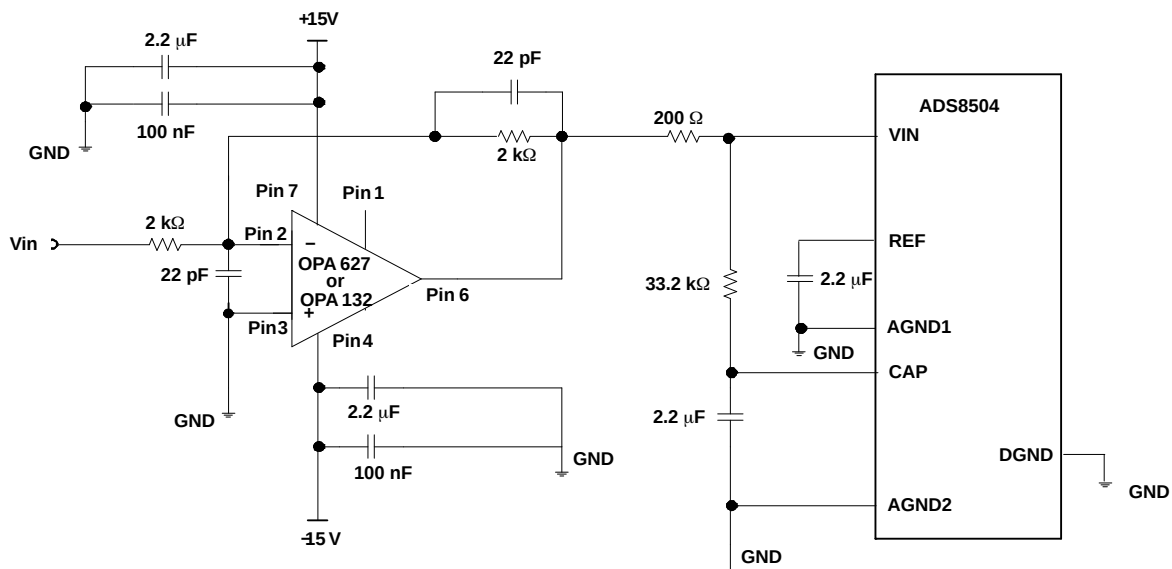
Figure 22. Typical Driving Circuitry ( \pm 10 V, No Trim)
